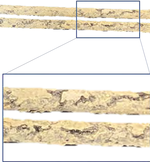
Limescale buildup on a water heater electric element caused by calcium bicarbonate
